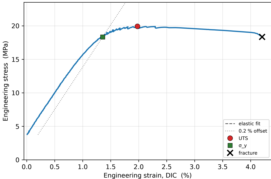
Stress-strain
